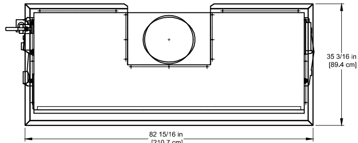
OUTDOOR TOP PANEL
